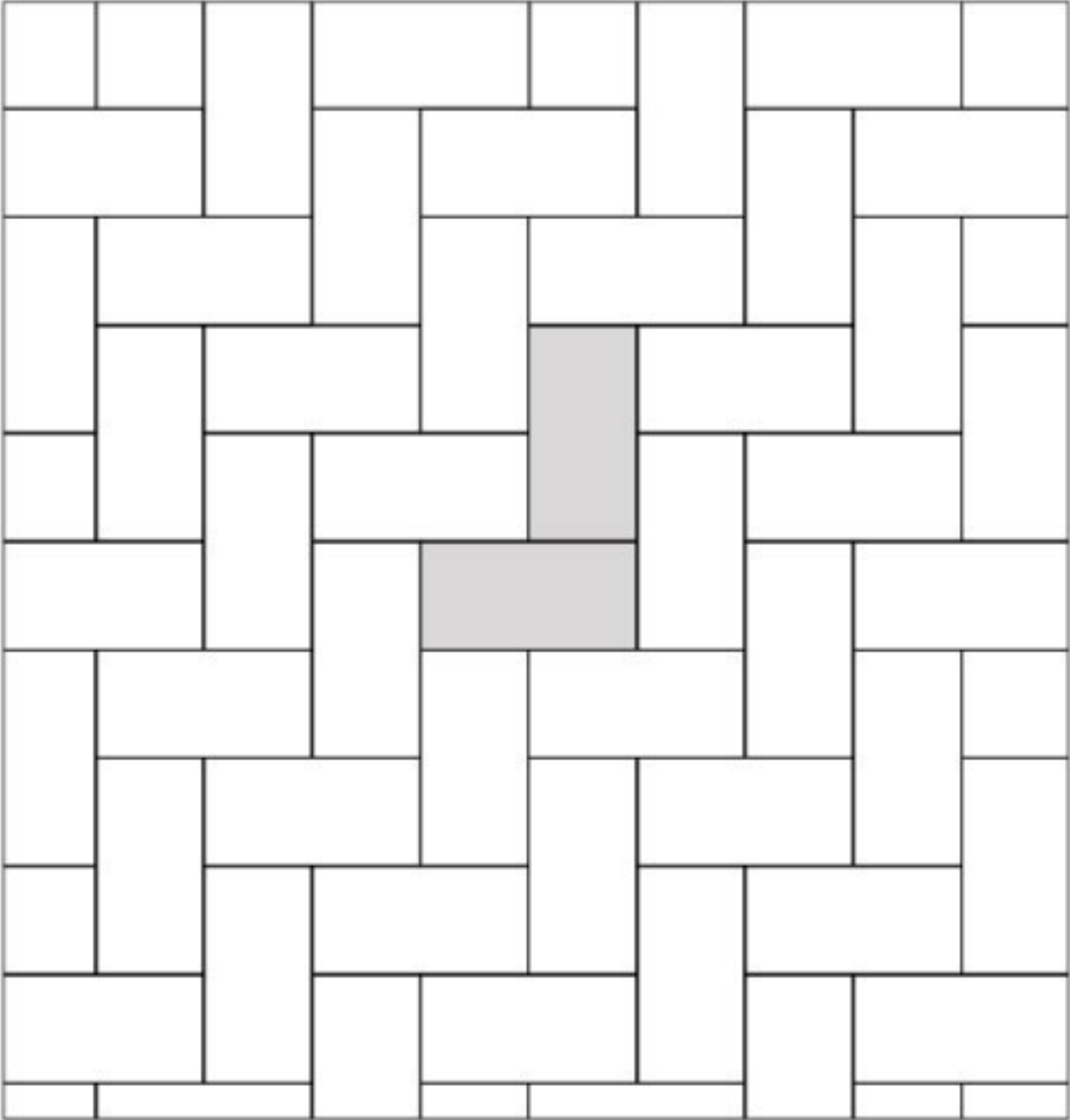
LAYING 16"x32" FOUR
