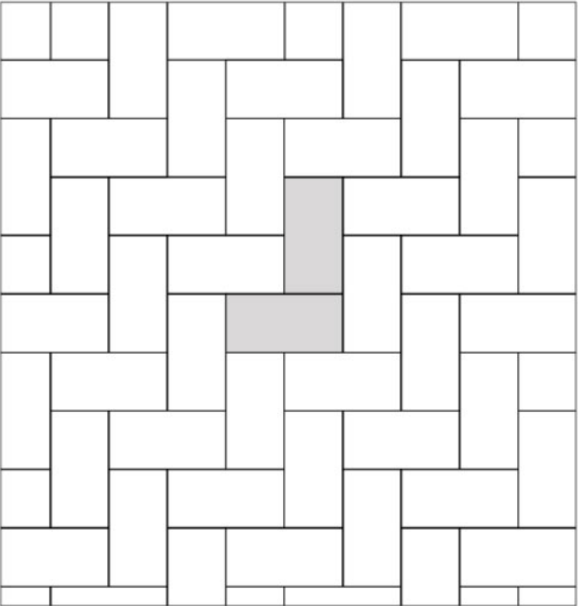
LAYING 12"x24" FOUR
