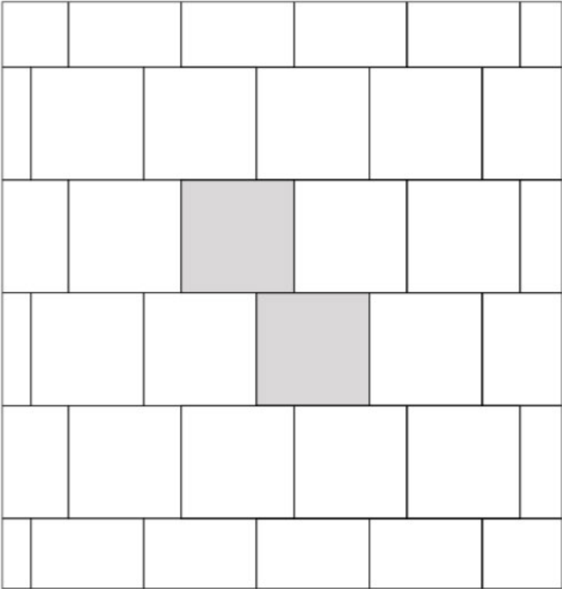
LAYING 24"x24" THREE
